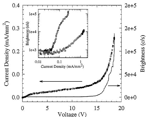
Fig. 5. Current density-voltage characteristics (○) and brightness-voltage characteristics of an ITO/PVK/PPyVP(COOC 12 H 25 ) 2 V/Al device. Inset shows a comparison between a single layer, ITO/PPyVP(COOC 12 H 25 ) 2 V/Al, device (□) and the bilayer device (○). The bilayer device is 10 times brighter at 10 times lower current density implying a 100 times improvement in efficiency.
