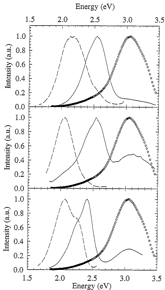
Fig. 3. Photoluminescence of (a) PPyVP(C 12 H 25 ) 2 V film (dashed line), PVK/PPyVP(C 12 H 25 ) 2 V bilayer film (solid line), PVK film (○) (b) PPyVP(COOC 12 H 25 ) 2 V film (dashed line), PVK/PPyVP(COOC 12 H 25 ) 2 V bilayer film (solid line), PVK film (○), and (c) strapped copolymer film (dashed line), PVK/strapped copolymer bilayer film (solid line), PVK film (○).
