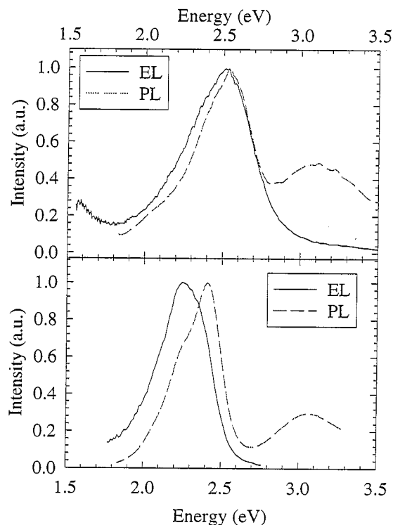
Fig. 4. Electroluminescence (solid lines) for a (a) ITO/PVK/PPyVP(COOC 12 H 25 ) 2 V/Al device and a (b) ITO/PVK/strapped copolymer/Al device. Photoluminescence (dashed lines) for bilayer films of PVK and (a) PPyVP(COOC 12 H 25 ) 2 V and (b) strapped copolymer.
