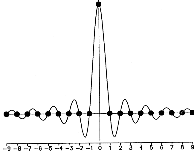
Figure 1.4: The general interpolating function \phi(t) for the same sampling frequency as in Fig 1.2.
