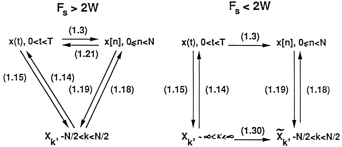
Figure 1.2: A. Relation between the continuous time signal x(t) , the sampled signal x[n] and the Fourier coefficients X_k when F_s is above Nyquist's rate. Numbers refer to formulas in the text. B. Same as A. when F_s is below Nyquist's rate. \tilde{X}_k refers to the Fourier coefficients of the sampled signal which now differ from those of x(t) .
