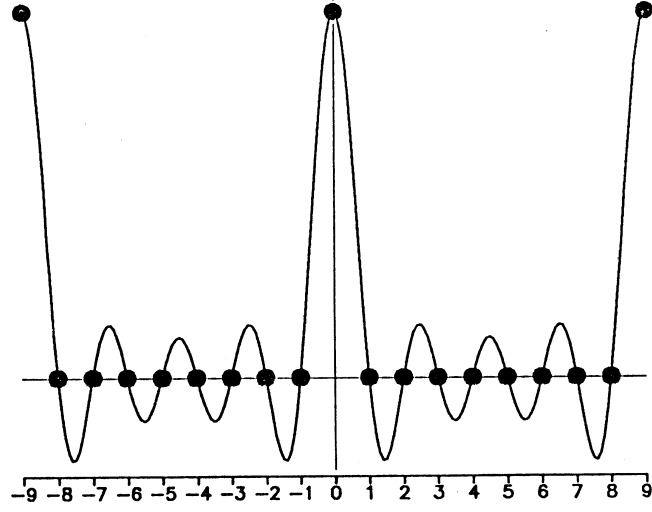
Figure 1.3: The periodic interpolating function \phi_N(t) for N = 9 and F_s = 1 .
