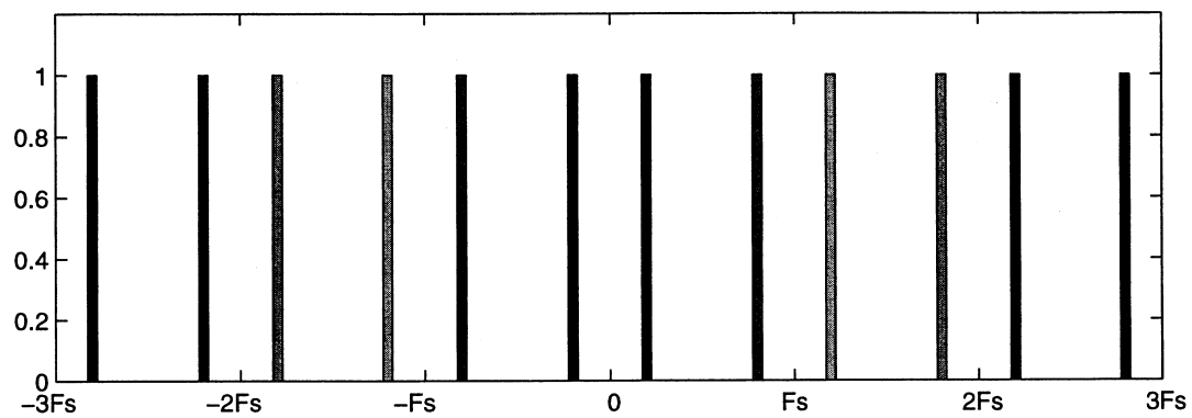
Figure 1.14: Sampling of an analog sine wave, F_s = 5F
