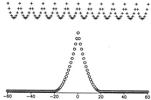
Figure 1.7: Effects of sampling at 4 different frequencies on the spectrum of a periodic signal with 39 components. Crosses show the Fourier coefficients of the sampled signal, circles those of the continuous-time signal.
