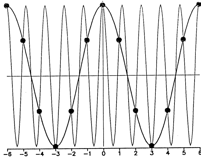
Figure 1.5: Aliasing: Two sinewaves with different frequencies that have the same samples.
