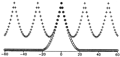
Figure 1.7: Effects of sampling at 4 different frequencies on the spectrum of a periodic signal with 39 components. Crosses show the Fourier coefficients of the sampled signal, circles those of the continuous-time signal.
