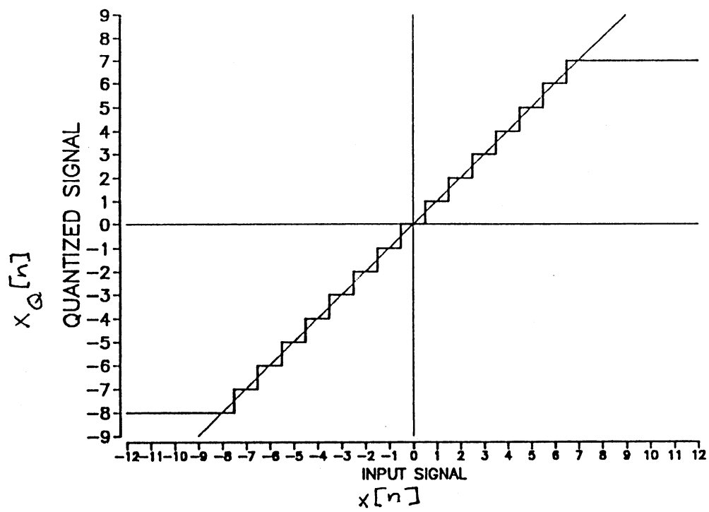
Figure 1.8: Input-output function for a 4-bit quantizer.
