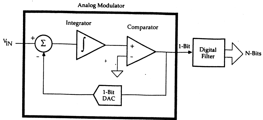
Figure 1.10: (from Analog Devices ) Block diagram of sigma-delta modulation A/D system.
